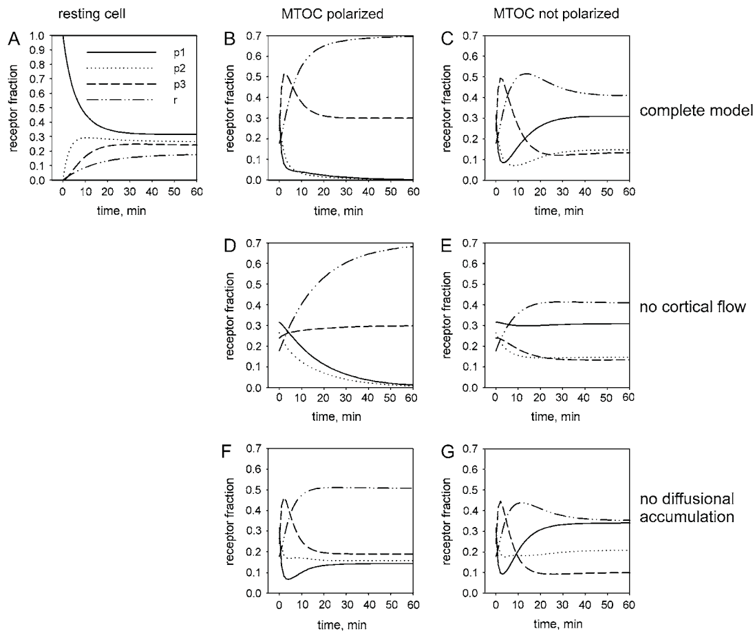
FIGURE 2 Redistributive of TCR between the intracellular pool ( r ) and the different regions on the PM ( p_1 , p_2 , p_3 ), of which p_3 corresponds to the immunological synapse, p_1 to the opposite pole of the cell, and p_2 to the equatorial region. The figure parts (A–G) correspond to Models A–G, the kinetic diagrams of which are shown in corresponding panels of Fig. 1. Part A here contains the curve labels, and also shows the equilibration in an unstimulated cell from an arbitrary initial condition, demonstrating how the steady state is reached which is used as the initial condition in all the models of the stimulated cell (B–G). Parts B–G show redistribution in a stimulated cell, in the different models and situations as labeled.
